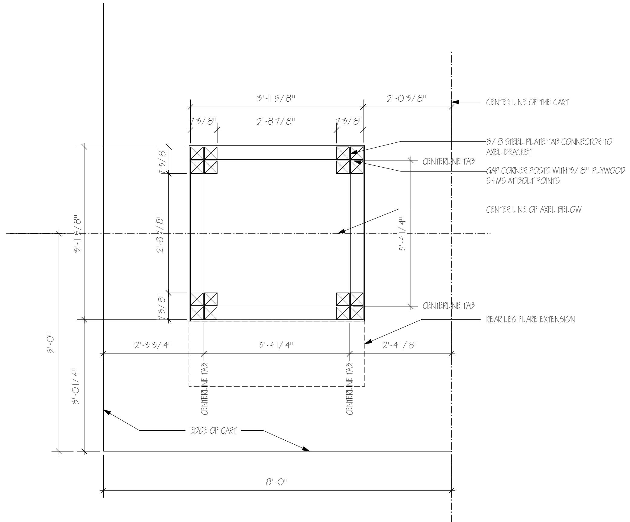
1 Leg Framing Plan Scale: 3/4" = 1'-0"
