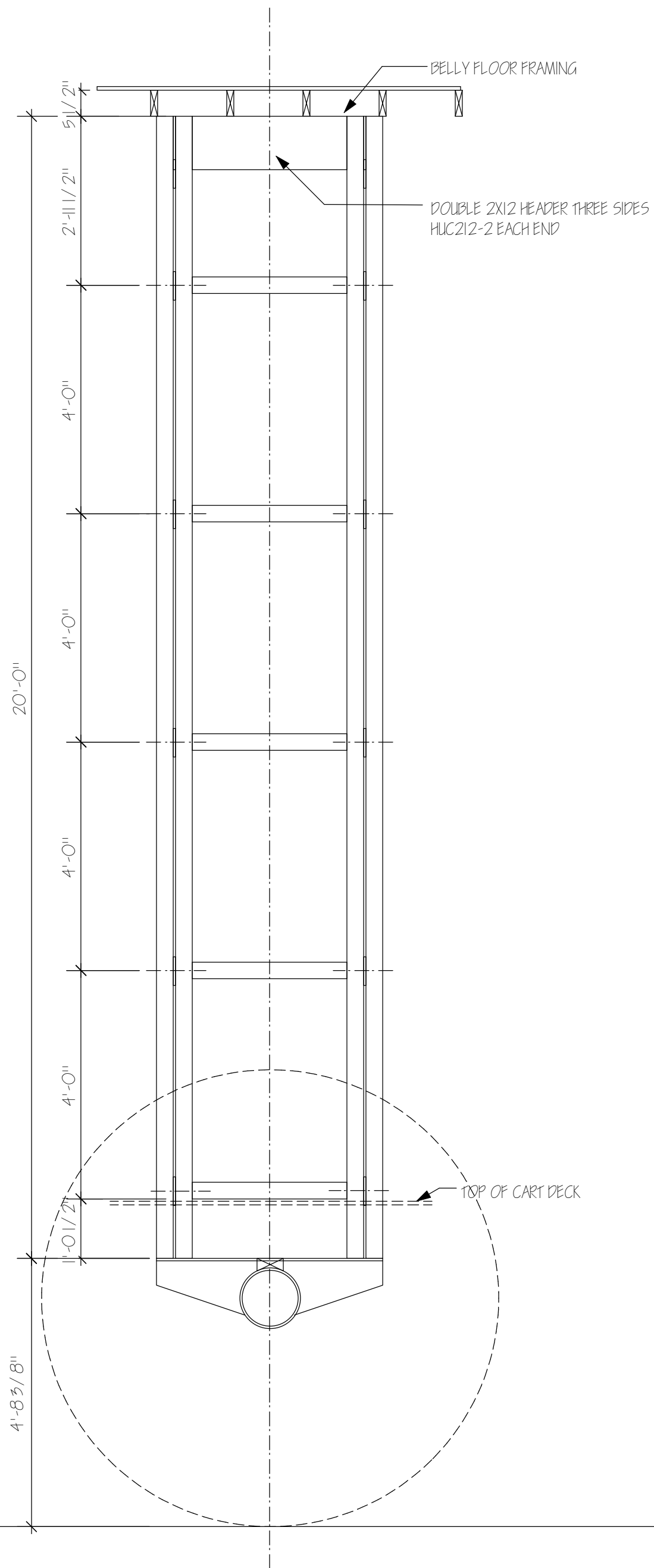
1 Leg Framing Elevation - Outside Scale: 1/2" = 1'-0"
