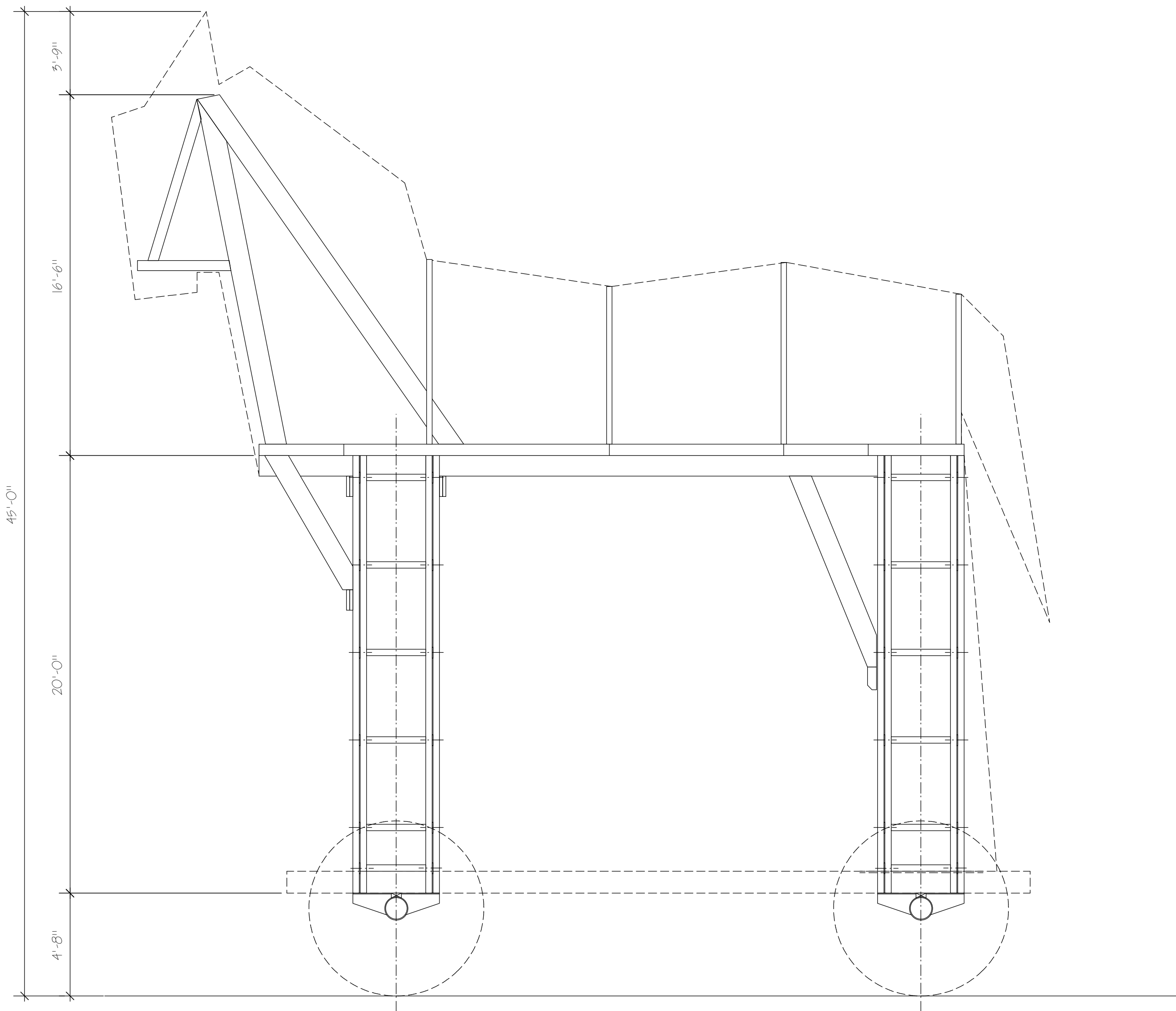
1 Trojan Horse Framing Elevation Scale: 1/4" = 1'-0"
